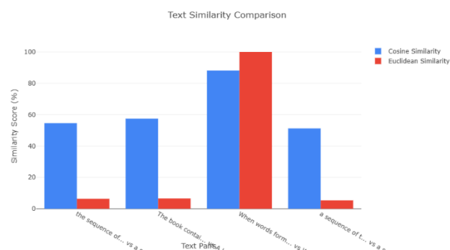
Figure 13. Comparison of Similarity Scores Between Subsequence Pairs using HTM SDRs
