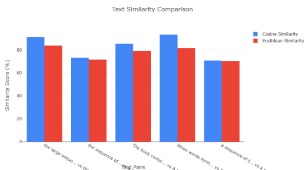
Figure 11. Comparison of Similarity Scores Between Subsequence Pairs using Basic SDRs
